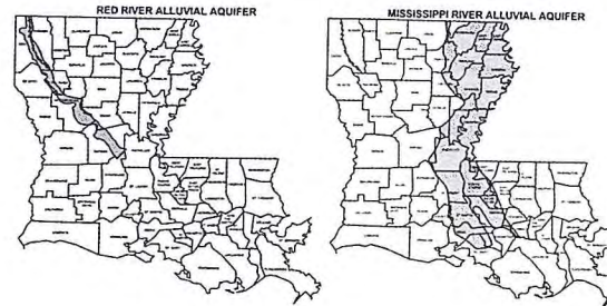
Unconsolidated (sand and gravel) alluvial aquifer systems in Louisiana which may be unsafe for domestic water well use. 2
